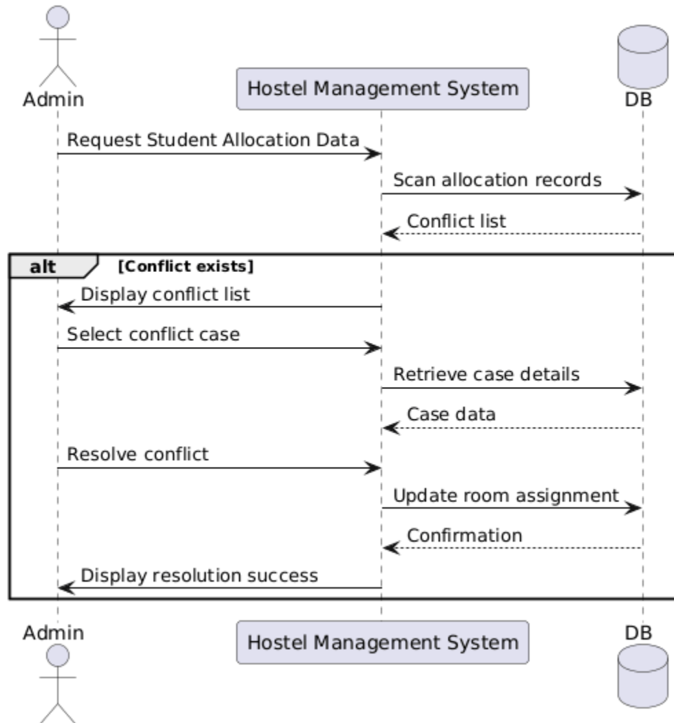
Figure 1.13: Sequence Diagram for Check for Allocation Conflict & Resolve Conflict
