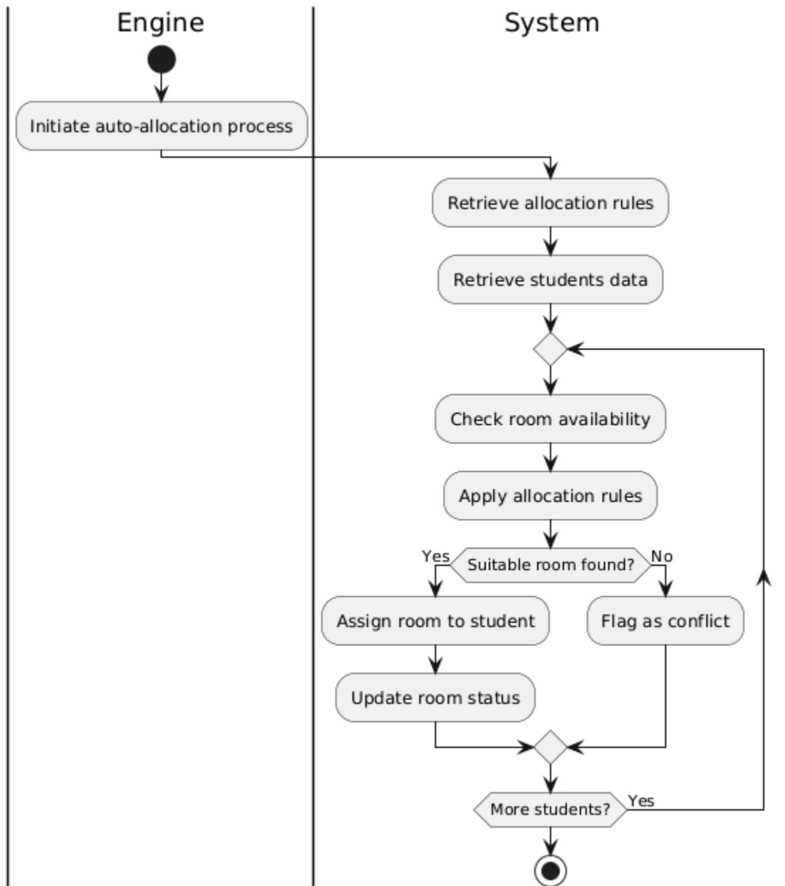
Figure 1.10: Activity Diagram for Auto-Allocate Room
