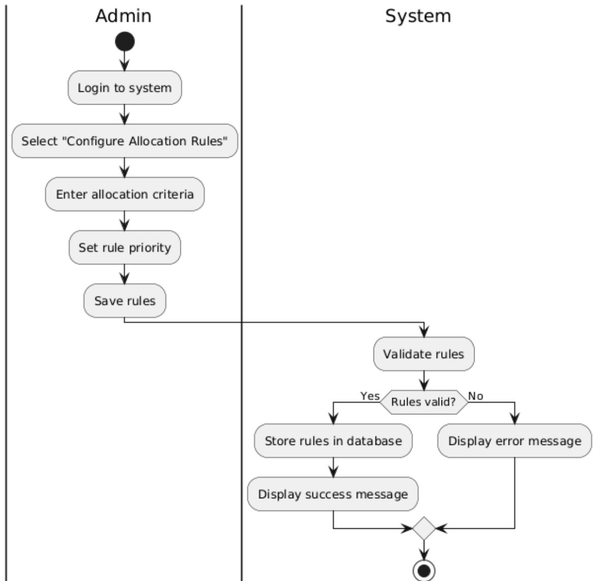
Figure 1.6: Activity Diagram for Configure Allocation Rules
