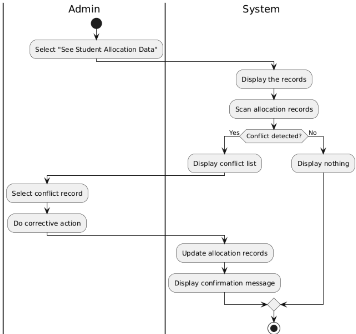
Figure 1.9: Activity Diagram for Check for Allocation & Resolve Conflict
