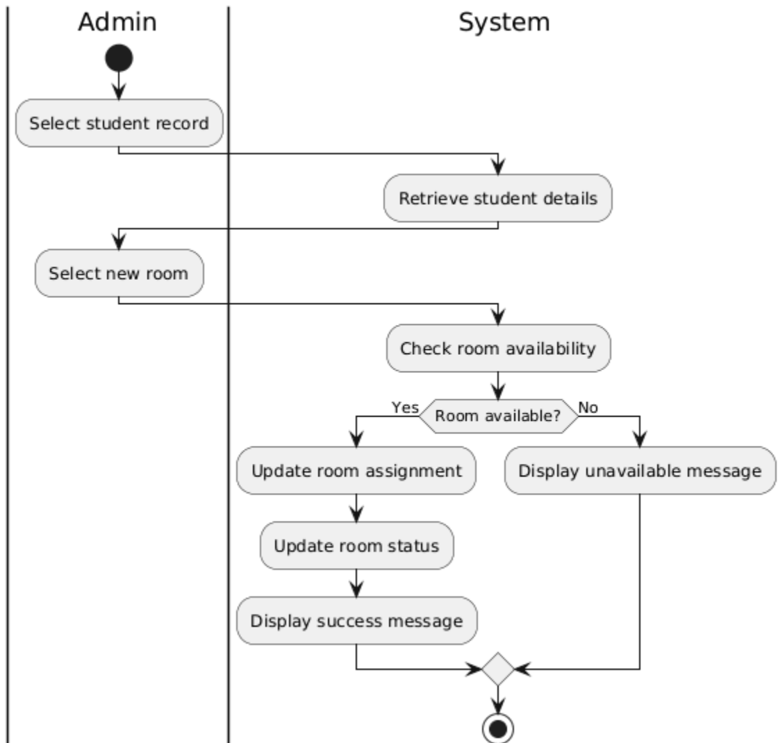
Figure 1.7: Activity Diagram for Modify Room Assignment
