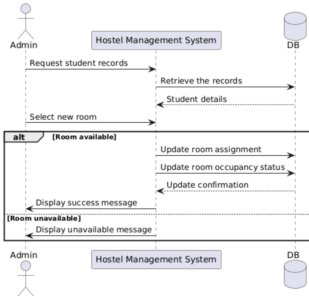
Figure 1.12: Sequence Diagram for Modify Room Assignment
