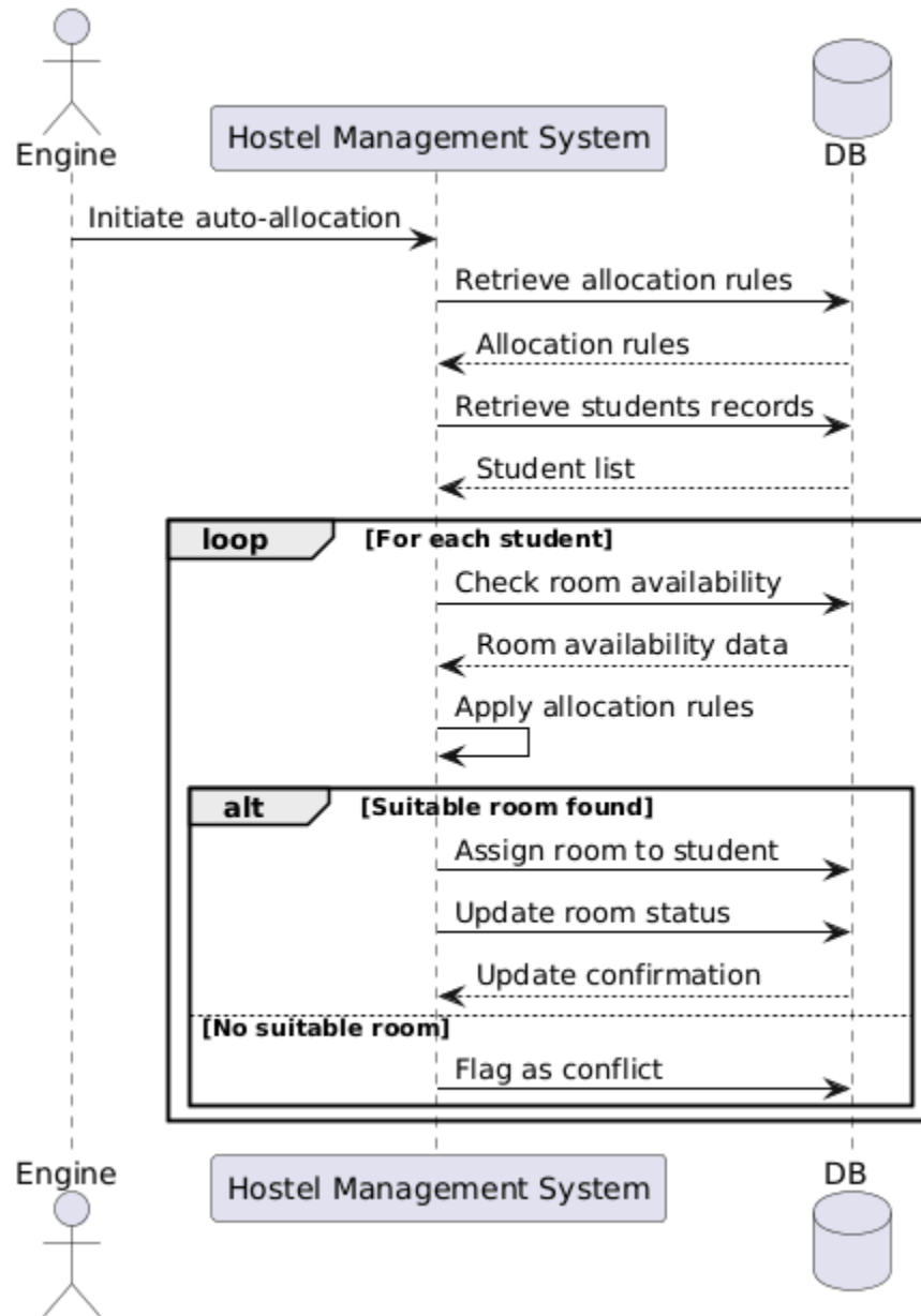
Figure 1.14: Sequence Diagram for Auto-Allocate Room
