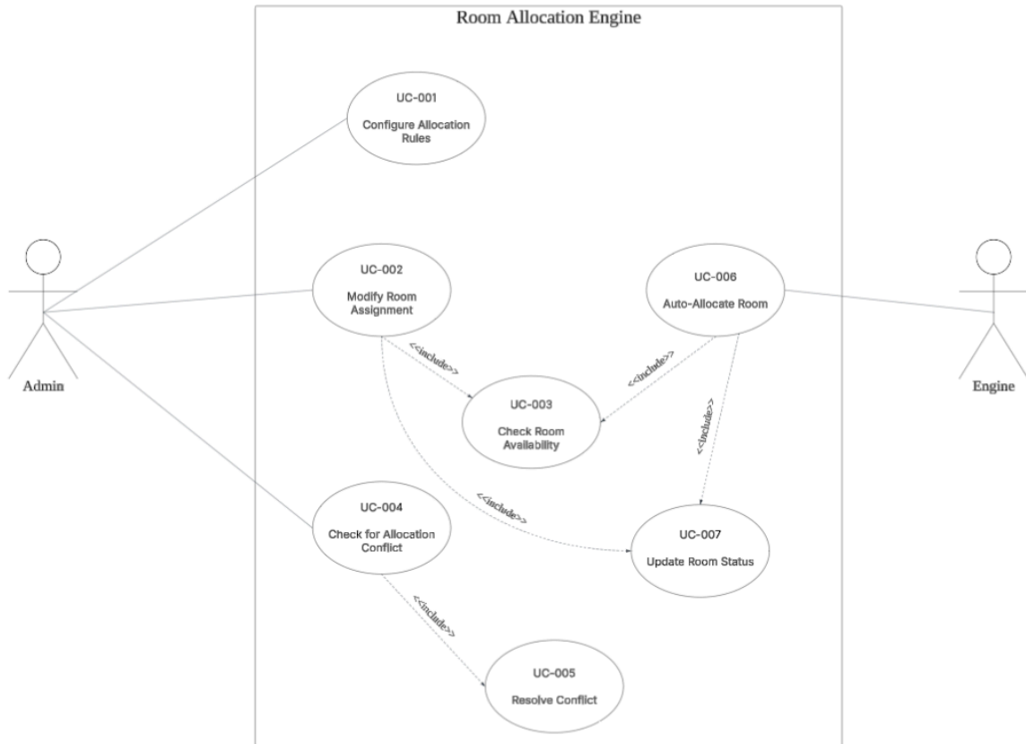
Figure 1.5: Use Case Diagram for Room Allocation Engine
