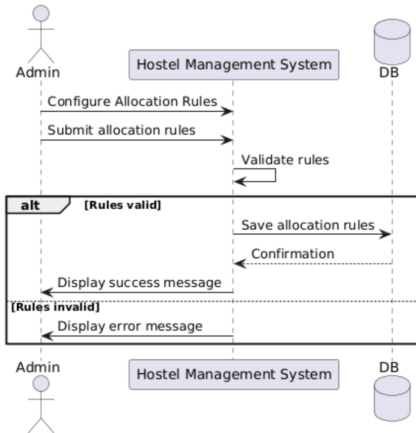
Figure 1.11: Sequence Diagram for Configure Allocation Rules
